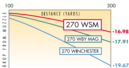
Drop from muzzle, 130 gr bullet
