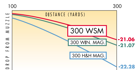
Drop from muzzle, 180 gr bullet
